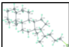
Fig. 1. Thermal ellipsoid plot (Barbour, 2001) of \text{C}_{24}\text{H}_{41}\text{Br} at the 70% probability level. Hydrogen atoms are drawn as spheres of arbitrary radius.
